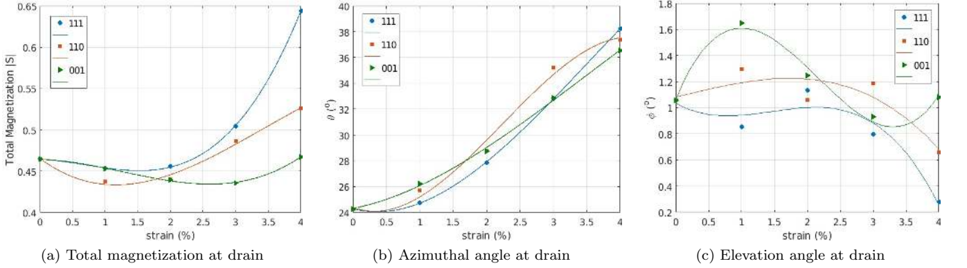
FIG. 14. Steady state magnetization showing total magnetisation (a), at drain as a function of strain along different axis ( x -injection, V_D = V_G = 0.9 V) with nonlinear spline fits shown by lines to serve as a guide to the eye in elucidating trends in the data.
