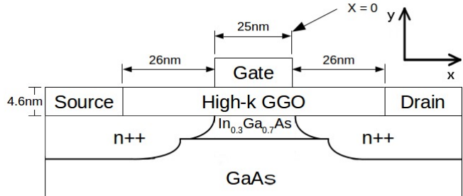
FIG. 3. Cross section of the 25 nm gate length, n -channel \text{In}_{0.3}\text{Ga}_{0.7}\text{As} MOSFET.
