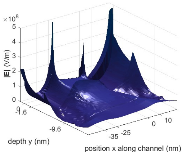
FIG. 9. Steady-state electric field \|\mathbf{E}\| in the device for one run of Monte Carlo simulator with V_G = 0.9 V and V_D = 0.5 V. The electric field is non-uniform, concentrated in the channel and near the electrodes, with large fringe fields at electrode boundaries.
