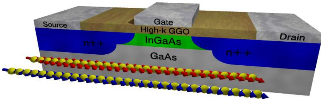
FIG. 1. 3D model of the studied \text{In}_{0.3}\text{Ga}_{0.7}\text{As} MOSFET showing spin polarization of electrons along n -channel with 4% strain in the [001] direction (Red) and unstrained (Dark Blue).
