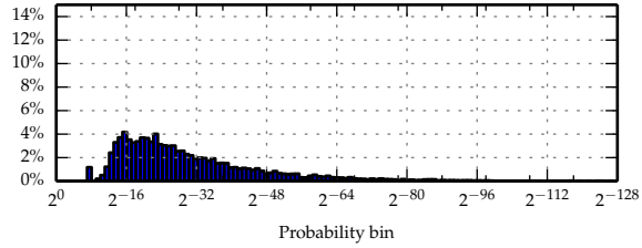
(b) 4-grams.
