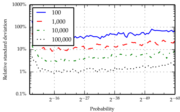
Figure 3: Estimation uncertainty while varying sample size. Supporting the result from Theorem 2, estimates converge as the sample size grows.
