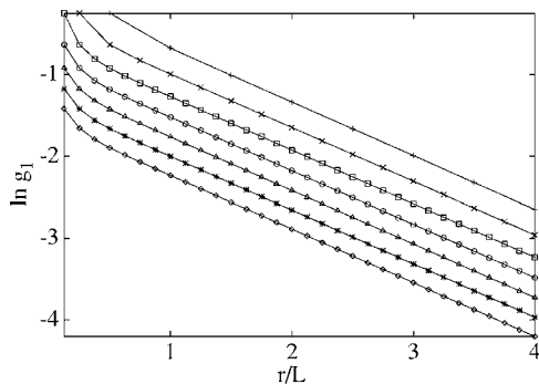
FIG. 11. Logarithm of the order parameter g_1(r) for the square-lattice bond-percolation model at criticality vs the scaled distance r/L to the first layer of the cylinder. The data points + , \times , \square , \circ , \triangle , * , and \diamond represent system sizes L=8, 16, 32, 64, 128, 256 , and 512 , respectively.
