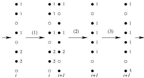
FIG. 1. Illustration of the cluster construction for the newly added layer without the help of the “linkage” technique. This example applies to linear size L=8 , and free boundary conditions are imposed in the vertical direction.
