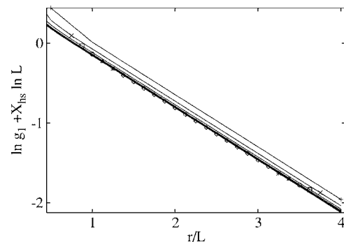
FIG. 12. Logarithm of the order parameter g_1(r) for the square-lattice bond-percolation model at criticality vs the scaled distance r/L . The quantity X_{hs} used to the rescaling of the vertical axis is the surface magnetic dimension at the ordinary phase transition X_{hs}^{(o)}=1/3 . The data points + , \times , \square , \circ , \triangle , * , and \diamond represent system sizes L=8, 16, 32, 64, 128, 256 , and 512 , respectively.
