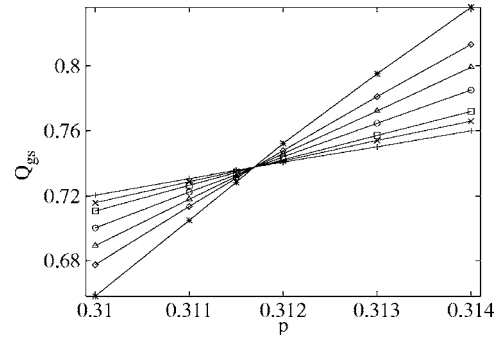
FIG. 10. Surface ratio Q_{gs} for the simple-cubic site-percolation model vs the site-occupation probability. The data points +, ×, □, ○, △, ◇, and * represent system sizes L=16,20,24,32,40,48 , and 64, respectively.
