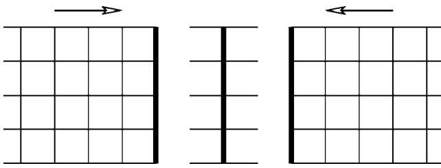
FIG. 3. Illustration of the sampling of bulk quantities. The thick solid lines represent the two free surfaces of the simulated strips and a newly inserted layer of randomly distributed occupied and empty sites, respectively. These layers are “glued” together by adding horizontal bonds.
