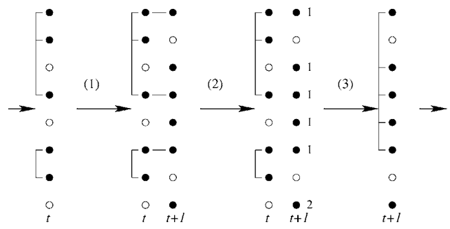
FIG. 2. Illustration of the cluster construction for the newly added layer with the help of the “linkage” technique. This example applies to linear size L=8 , and free boundary conditions are imposed in the vertical direction.
