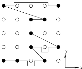
FIG. 4. Illustration of a cluster linkage on a two-dimensional layer of the cylinder L^2 \times \infty . The layer is a square lattice with L = 5 , with periodic boundary conditions in both the x and y directions.
