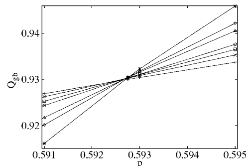
FIG. 6. Bulk ratio Q_{gb} for the square-lattice site-percolation model vs the site-occupation probability. The data points + , \times , \square , \circ , \triangle , \diamond , and * represent system sizes L = 16, 24, 32, 40, 64, 80 , and 120 , respectively.
