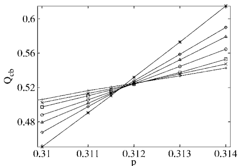
FIG. 9. Bulk ratio Q_{cb} for the simple-cubic site-percolation model vs the site-occupation probability. The data points +, ×, □, ○, △, ◇, and * represent system sizes L=16,20,24,32,40,48 , and 64, respectively.
