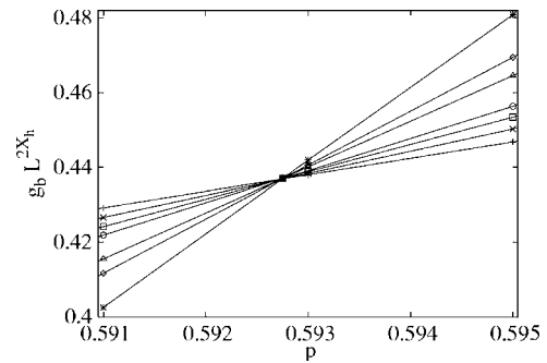
FIG. 5. Scaled magnetic bulk correlation L^{2X_h}g_b(L/2) for the square-lattice site-percolation model vs the site-occupation probability. The bulk magnetic scaling dimension X_h is equal to 5/48 . The data points + , \times , \square , \circ , \triangle , \diamond , and * represent system sizes L = 16, 24, 32, 40, 64, 80 , and 120 , respectively.
