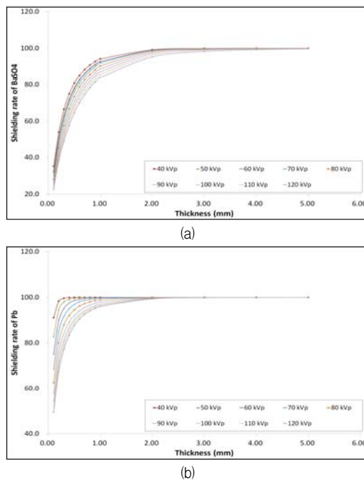
Fig. 3. shielding rate as a function of material thickness (a) Barium compound and (b) Lead.
