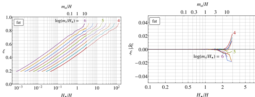
Figure 21: Left: The scaling parameter \xi as a function of time when the axion mass is turned on at different \log_\star \equiv \log(m_r^*/m_a^*) (solid lines), and for m_a = 0 throughout with the same initial condition (dashed lines). The x-axis is normalized with H_\star , so it can be seen that regardless of \log_\star , \xi is unaffected by the mass before H = H_\star . Right: The relative difference between the results for \xi with and without a non-zero axion mass, \delta\xi/\xi , as a function of time. We define \delta\xi \equiv (\xi - \xi_{m_a=0}) , and \xi_{m_a=0} is the string length in a simulation with m_a = 0 throughout. For all values of \log_\star tested the effect of a non-vanishing axion mass is smaller than percent for H > H_\star .
