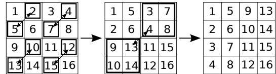
Figure 2: Efficient matrix transposition of a 4 \times 4 matrix using Eklundh’s algorithm.
