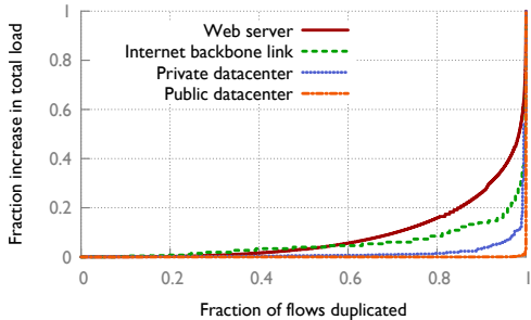
Figure 1: Overhead of duplicating traffic.
