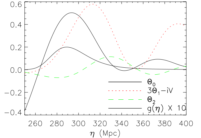
FIG. 5 (color online). \Theta_0^{(1)} , 3\Theta_1^{(1)} - i\nu^{(1)} , and \Theta_2^{(1)} as a function of \eta for wave number k = 0.1 \text{ Mpc}^{-1} . Note that at small scales 3\Theta_1^{(1)} - i\nu^{(1)} becomes comparable to \Theta_0^{(1)} , but its contribution to the bispectrum is suppressed because it is weighted by the derivative of spherical Bessel function. See also Eq. (10) and Fig. 3 in KW09.
