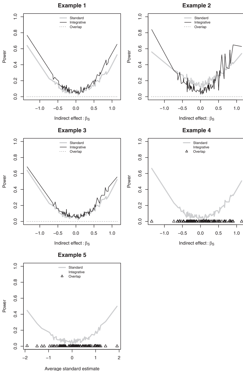
Figure 1. Average power curves for linear outcomes. Integration, proposed method; standard, standard univariate regression analysis; overlap, overlap method.
