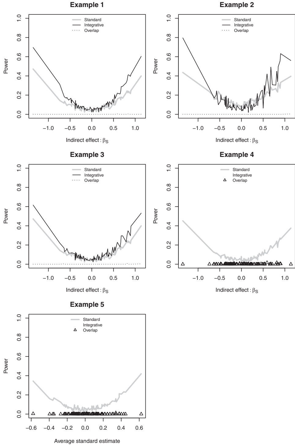
Figure 2. Average power curves for binary outcomes. Integration, proposed method; standard, standard univariate regression analysis; overlap, overlap method.
