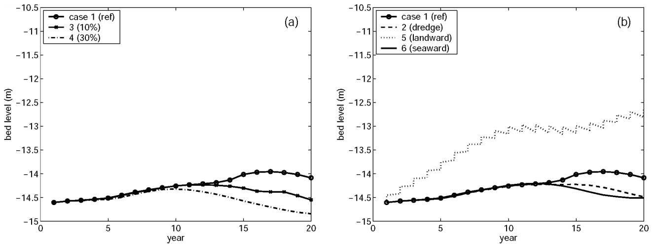
Figure 6.8: Evolution during 20 years of mean channel depth around dumping location B for different dredging and dumping scenario's. (a) shows an ongoing shoaling of the area due to dumping at this location, which is enhanced when the dumped volume is increased. (b) shows the influence of the dredging activities in the nearby threshold area as an increase of channel depth with respect to the reference case. The depth increase is similar for only dredging (Case 2, dashed) as for dredging and dumping in the seaward cell (Case 6, solid). Channel erosion is largest for Case 5 (dotted), in which the material is dumped in the channel opposite to this location.
