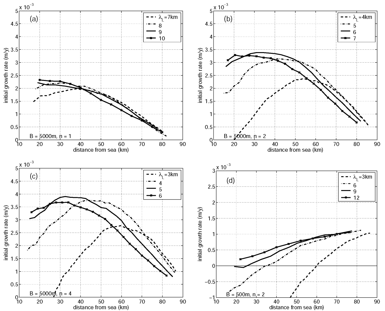
Figure 4.4: Initial growth of prevalent perturbations in wide basin ( B = 5 km) for (a) \lambda_T = 10 km (first mode), (b) \lambda_T = 5 km (second mode), (c) \lambda_T = 2.5 km ( n = 4 ) and (d) in the narrow basin for \lambda_T = B = 500 m (second mode). Note that the y -axis scale differs.
