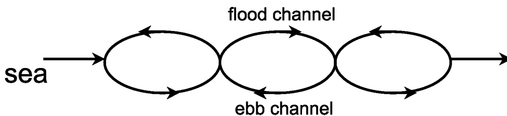
Figure 6.1: Sketch of serially coupled morphological cells (after Winterwerp et al., 2001).
