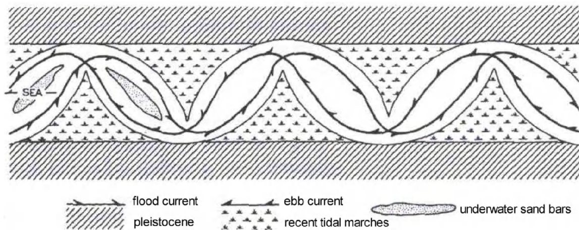
Figure 2.4: Sketch of meandering tidal channel system by Ahnert (1960).
