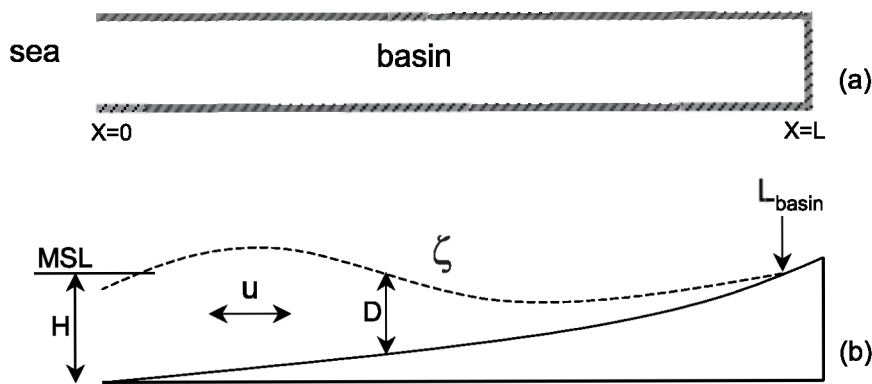
Figure 3.1: The top view (a) and side view of an idealised geometry as used in the experiments. The symbols are explained in the text. Here MSL denotes the mean sea level.
