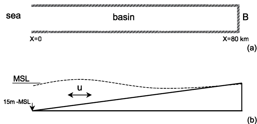
Figure 5.1: Upper panel: top view of estuary. Lower panel: side view of estuary.
