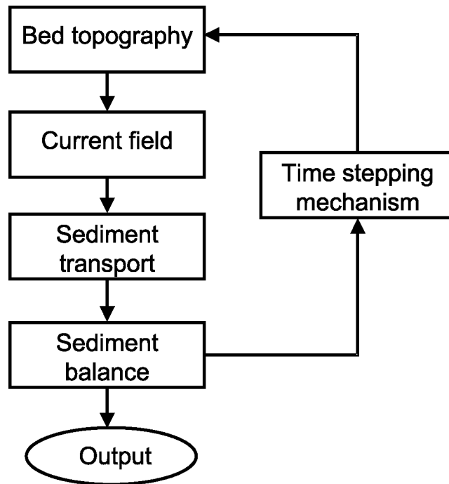
Figure 2.1: Model scheme of process-based morphological model, showing time-loop of modules (adapted from De Vriend and Ribberink, 1996)
