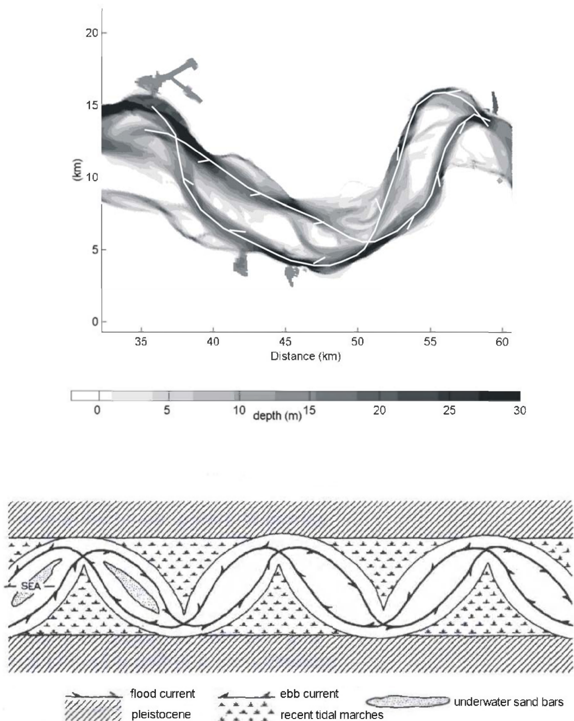
Figure 5.5: (a) Section of the Western Scheldt estuary, the Netherlands, 1996. The trajectories indicate the direction of the residual velocity. (b) Sketch of meandering channel system by Ahnert (1960).
