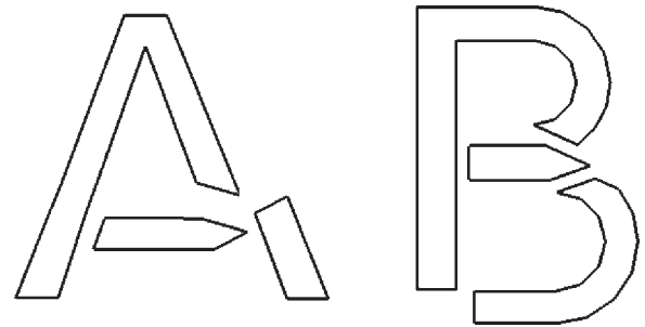
Figure 6. Letters A and B are decomposed into three equivalent patches.
