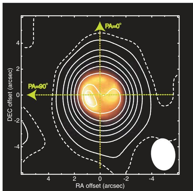
Figure 2. Total flux intensity map in the ^{12}\text{CO } J = 3-2 line superimposed on the mid-infrared 12.5 \mu\text{m} image taken from Kwok et al. (2002). The contour levels are 3, 19, 35, 67, 83, 99, and 105\sigma , and the 1\sigma level corresponds to 4.80 \times 10^{-2} \text{ Jy beam}^{-1} . The dashed contour correspond to -3\sigma . The FWHM beam size is located in the bottom right corner. The origin of the coordinate corresponds to the phase center. The dotted green arrows indicate the directions along which the p-v cuts shown in Figure 4 were taken.
