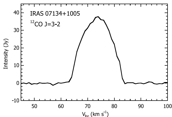
Figure 1. ^{12}\text{CO } J = 3-2 total flux line profile.
