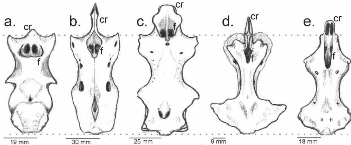
FIG. 4. – Neurocranium of (a) Centroscyllium granulatum (42 cm LT), (b) Deania calcea (80.5 cm LT), (c) Squalus acanthias (68 cm LT), (d) Halaelurus canescens (63 cm LT) and (e) Schroederichthys chilensis (69 cm LT). Were cr: rostral cartilage; f: fontanel. Scale bar (in mm) is indicated in each photograph.
