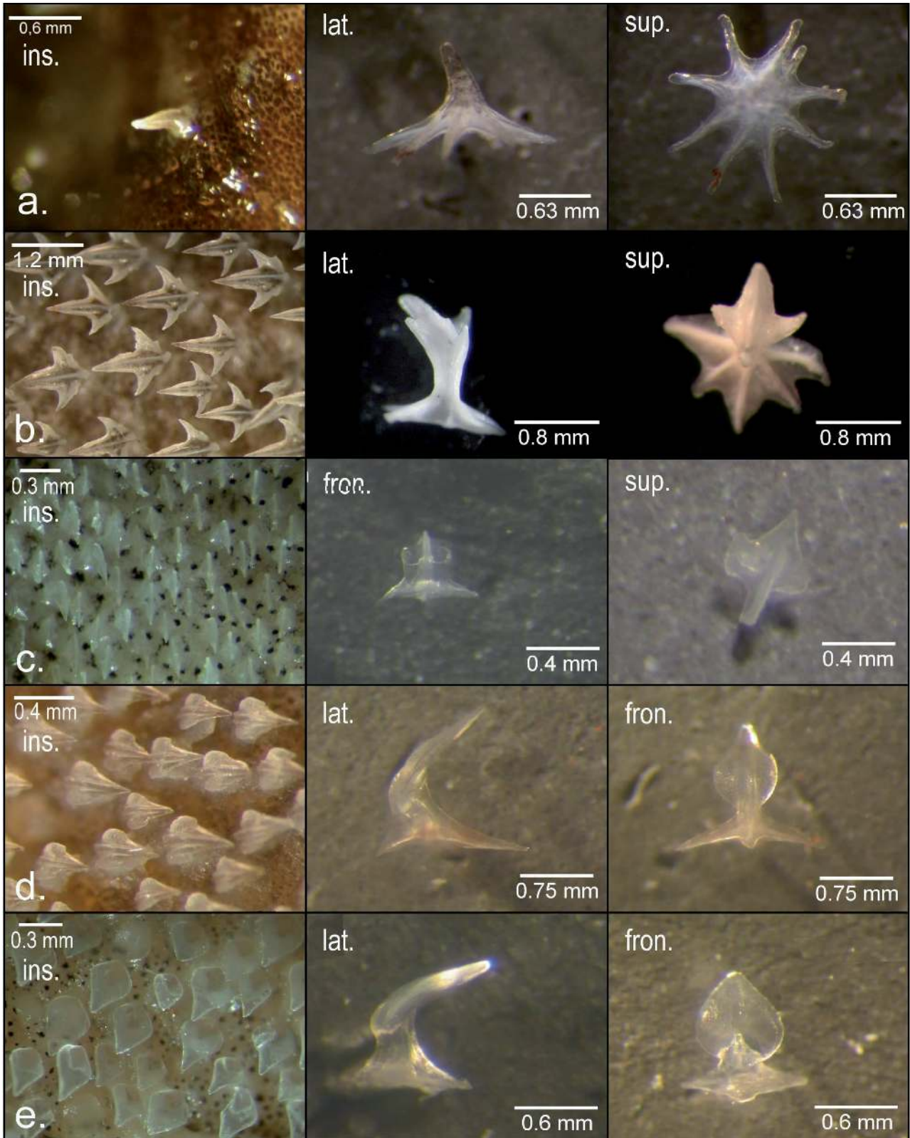
FIG. 3. – Post-pectoral ventral dermal denticles of (a) Centroscyllium granulatum ; (b) Deania calcea ; (c) Squalus acanthias ; (d) Halaehurus canescens ; and (e) Schroederichthys chilensis . ins: dermal denticle natural insertion in skin; lat: lateral view; fron: frontal view; up: top view. Scale bar (in mm) is indicated in each photograph.
