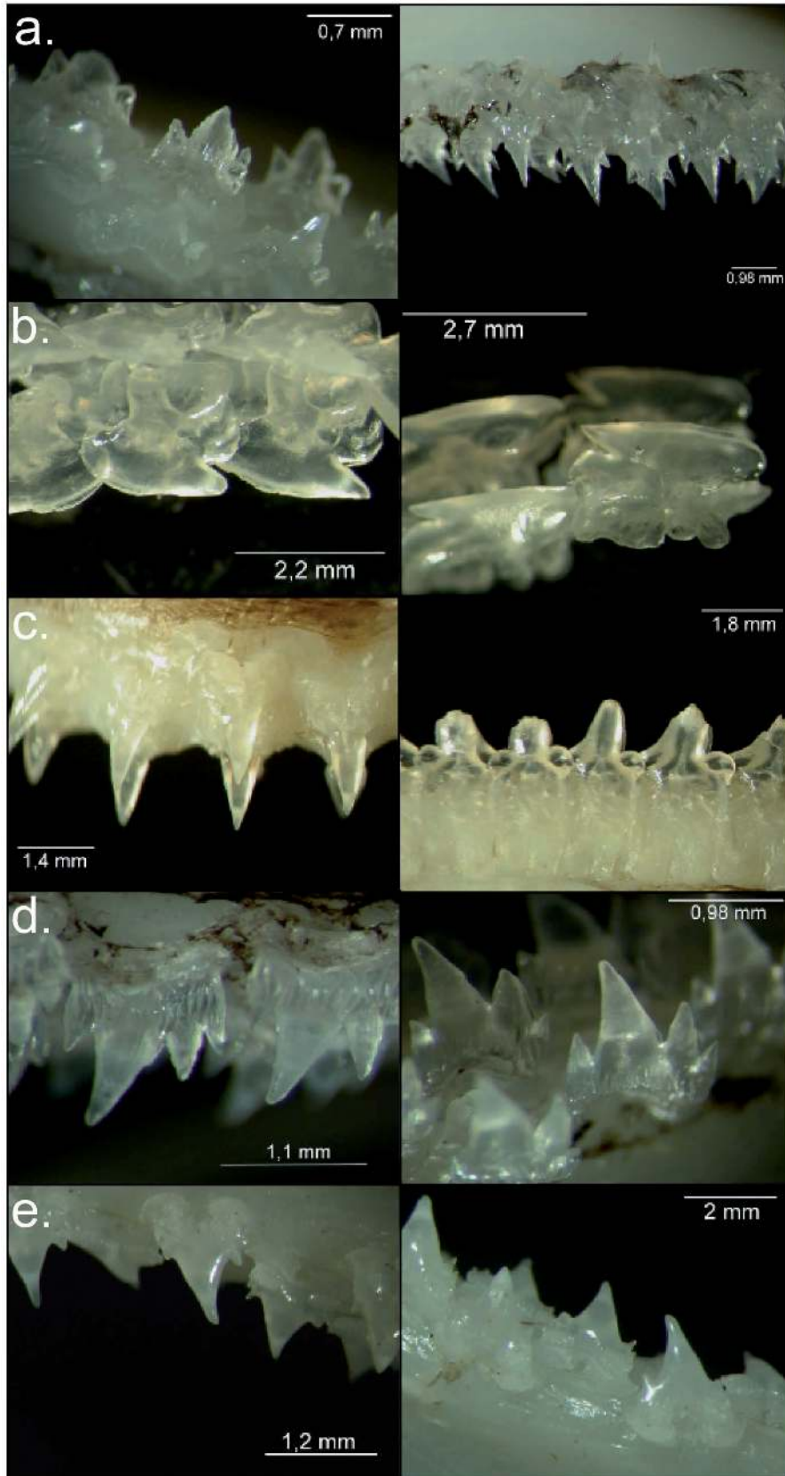
FIG. 2. – Frontal teeth of upper (left) and lower (right) jaws of (a) Centroscyllium granulatum ; (b) Squalus acanthias ; (c) Deania calcea ; (d) Halaelurus canescens ; and (e) Schroederichthys chilensis . Scale bar (in mm) is indicated on each photograph.
