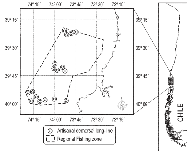
FIG. 1. – Sampling zone of the artisanal fisheries of Genypterus blacodes and Dipturus chilensis during 2005. Fishing trips and regional fishing zone are indicated
