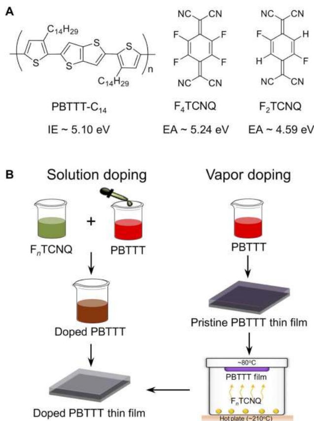
Fig. 1. Chemical structure and doping process. (A) Chemical structure of PBTTT and F_nTCNQ ( n = 2 or 4 ) and the corresponding IE or EA. (B) Solution and vapor doping routes used to achieve doped films.
