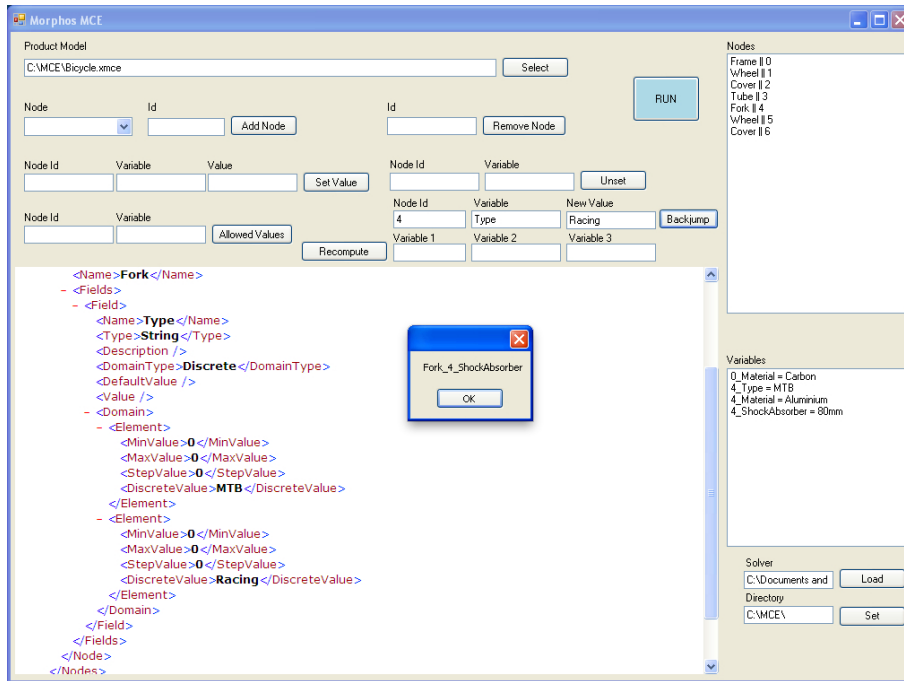
Figure 8: Taking advantage of the Backjump button and the related text fields Node Id , Variable , and New Value , the user chooses the new value for Fork, id=4.Type. The system computes a set of choices that have to be withdrawn and returns it through a message box.
