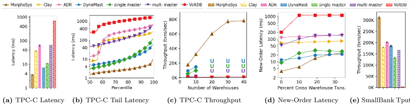
(a) TPC-C Latency (b) TPC-C Tail Latency (c) TPC-C Throughput (d) New-Order Latency (e) SmallBank Tput Figure 5: Performance results for the TPC-C and SmallBank workloads. In Figure 5c, U 's indicate that fully replicated systems (DynaMast, single-master and multi-master) were unable to run due to memory constraints.
