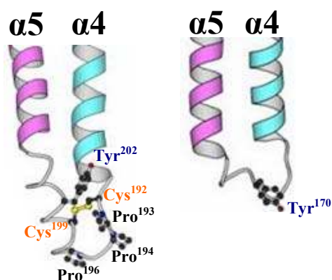
Fig. (2). Ribbon representations of the loop connecting \alpha4 and \alpha5 of two known structures: Cry4Aa (left) and Cry4Ba (right). The highly conserved aromatic residue (Tyr 202 for Cry4Aa, Tyr 170 for Cry4Ba) is shown in ball-and-stick in both interhelical loops. Three critical proline residues (Pro 193 , Pro 194 and Pro 196 ) and the unique disulphide bond between Cys 192 and Cys 199 are illustrated as ball-and-stick in the Cry4Aa \alpha4 - \alpha5 loop.
