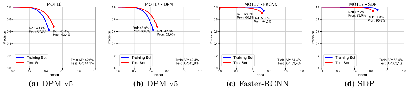
Fig. 4 The performance of three popular pedestrian detectors evaluated on the training (blue) and the test (red) set. The circle indicates the operating point (i.e. the input detection set) for the trackers of MOT16 and MOT17 (Color figure online)
