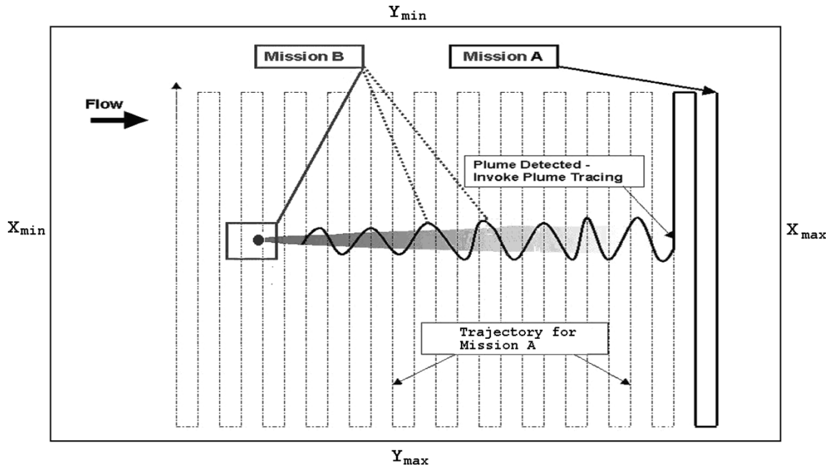
Fig. 1. Ideal plume tracing in the planning coordinate system. The solid black line indicates the actual AUV trajectory including preplanned (Mission A) and reactively planned (Mission B) portions. The circle indicates the chemical source. The flow is drawn positive to the right. The shaded cone emanating from the source depicts a highly simplified chemical plume.
