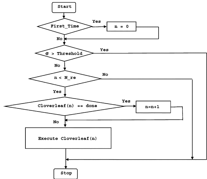
Fig. 8. Diagram for reacquire-plume behavior action.
