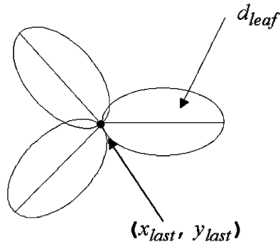
Fig. 7. Clover-leaf trajectory for the reacquire-plume behavior. The orientation of the trajectory in this figure assumes that the flow is from left to right. The maneuver is centered on the last detection point.
