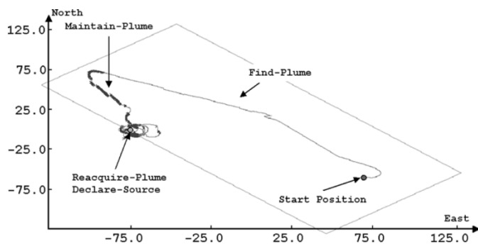
Fig. 12. CPT mission MSN010r2 for t in [80.4, 406.0] s. This time period includes find-plume, maintain-plume, reacquire-plume, and declare-source behaviors. The thick x's indicate locations where the chemical concentration was above threshold when the vehicle was at that location.
