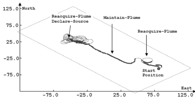
Fig. 10. AUV trajectory during plume tracing and source declaration for t in [480.3, 1190.6] s during mission MSN007r2. This time period includes maintain-plume, reacquire-plume, and declare-source behaviors. The thick x's indicate locations where the chemical concentration was above threshold when the vehicle was at that location.
