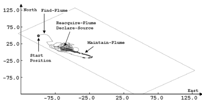
Fig. 11. CPT mission MSN008r1 for t in [60.3, 707.6] s. This time period includes find-plume, maintain-plume, reacquire-plume, and declare-source behaviors. The thick x's indicate locations where the chemical concentration was above threshold when the vehicle was at that location.
