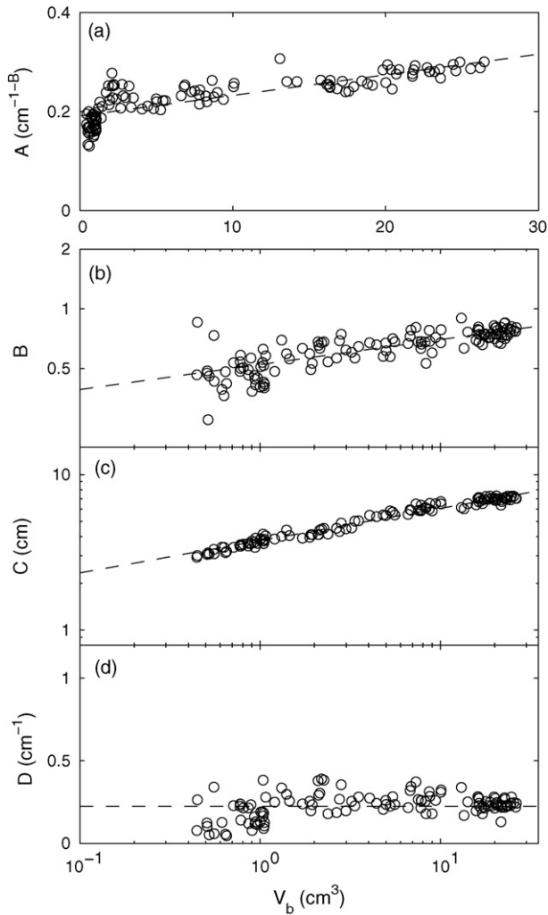
Fig. 6. The parameters A – D obtained from fits of the measured bubble profiles to Eq. (4) for a Carbopol concentration c = 1.8\% are plotted as a function of V_b in graphs (a)–(d), respectively. The uncertainties in the parameter values are typically in the order of the scatter in the data. In each case the dashed lines are fits to the data discussed in the text.
