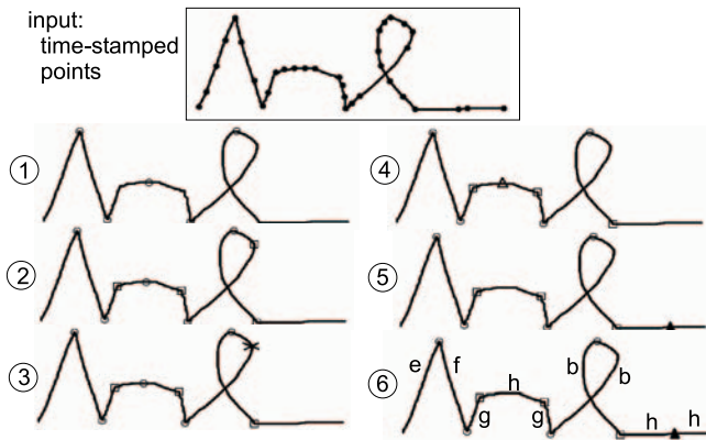
Figure 8: Tokenization consists of six steps: (1) Rough segmentation based on vertical direction of motion; (2) Corner detection; (3) Corner post-processing; (4) Merge colinear segments; (5) Identify pauses; (6) Token assignment.
