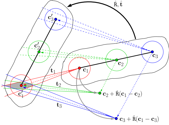
Figure 3. The shaded region is the intersection of three polyhedra located on where each camera sees, c'_1 , the centre of the first camera after a rigid motion. The shaded region is a feasible solution of the translation of this multi-camera system.
