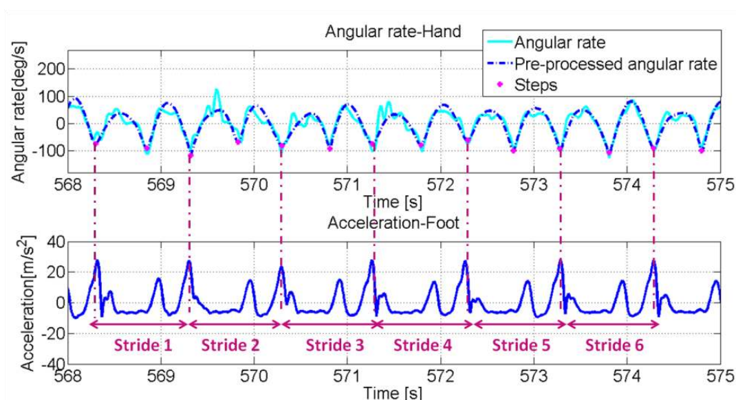
Figure 8. (Upper) Gyroscope signal (norm) recorded by the IMU in the swinging hand. The dots represent the detected step events. (Down) Accelerometer signal (norm) recorded by the IMU on the foot (the mean has been removed).
