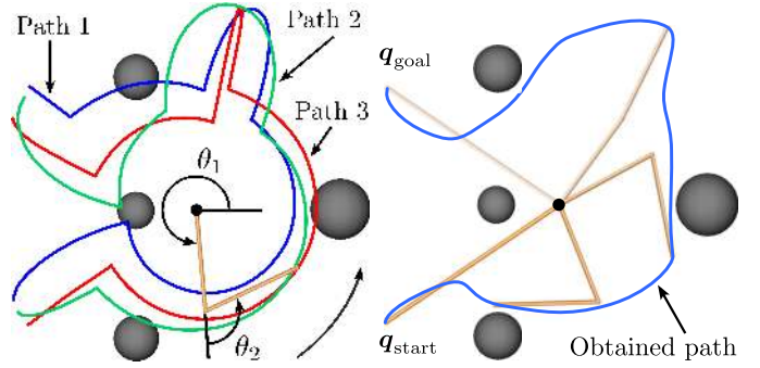
Fig. 4. 2-link planar manipulator problem: demonstrated paths (left) and obtained solution path (right).
