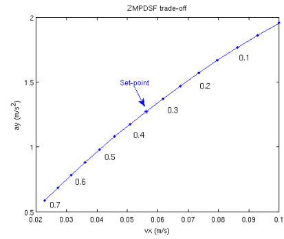
Fig. 4. Relation between average forward speed and maximum lateral acceleration of the CoM while the ZMPDSF parameter is modified. The values of this parameter are shown next to the curve. The value 0.35 for the ZMPDSF is chosen as the set-point for the experiments.
