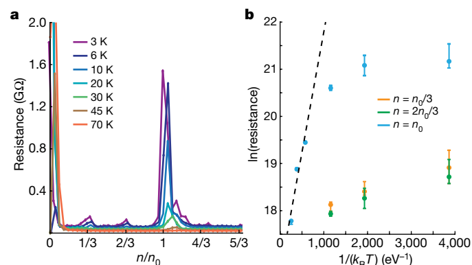
Fig. 3 | Temperature dependence of Mott and generalized Wigner crystal states. a , Resistance derived from ODRC measurements performed at temperatures between 3 K and 70 K. The Mott insulator state at n = n_0 is observable up to 45 K, and the generalized Wigner crystal states at n = n_0/3 and n = 2n_0/3 persist until 10 K. b , Plot of \ln(\text{resistance}) versus 1/k_B T for Mott (blue) and generalized Wigner crystal states (orange and green). Error bars correspond to the estimated experimental uncertainty in the extracted resistance values. The estimated thermal-activation gap for the Mott state is about 10 meV, which is found by fitting the data in b with a thermal-activation function (black dashed line).
