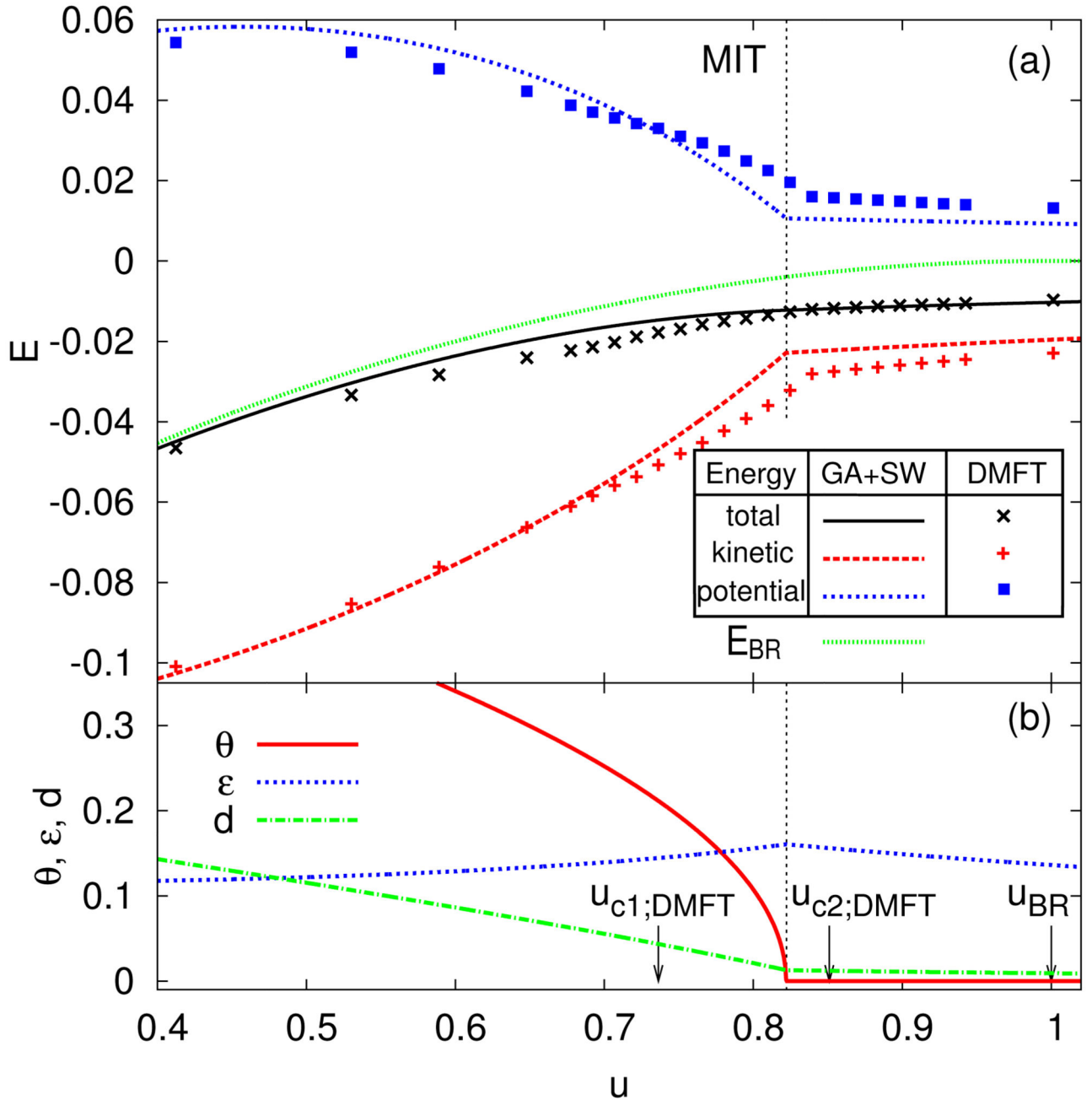
Fig. 1. (a) The equilibrium energy balance across the metal to insulator transition (MIT). For a comparison we have provided data points of the real energies from DMFT calculations [10]. Additionally for a reference we have also included the energy corresponding to the Brinkman-Rice result ( E_{BR} ) [2]. The transition takes place for quite similar critical interaction as for DMFT ( u_{c2;DMFT} ). Also, alike DMFT [3], potential and kinetic energies are characterized with the pronounced kinks while the total energy remains smooth. (b) The equilibrium values of \theta , \epsilon and d vs u across metal to insulator transition. We marked the
