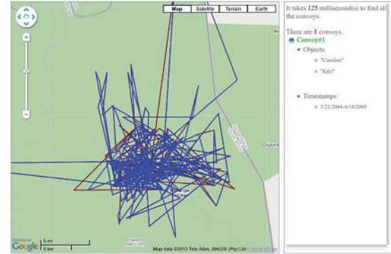
(b) one convoy discovered with min_o = m = 2 and min_t = k = 0.2
