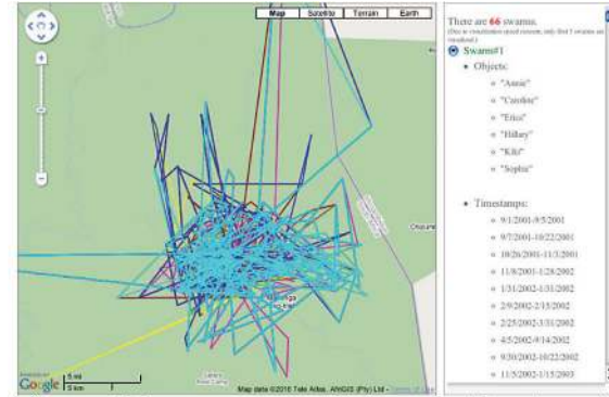
(a) one of the seven swarms discovered with min_o = 2 and min_t = 0.5
