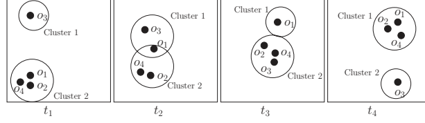
Fig. 6. Snapshots of object clusters at t_1 to t_4 .
