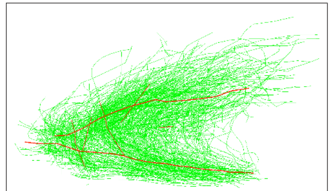
Figure 5: Trajectory Clustering
