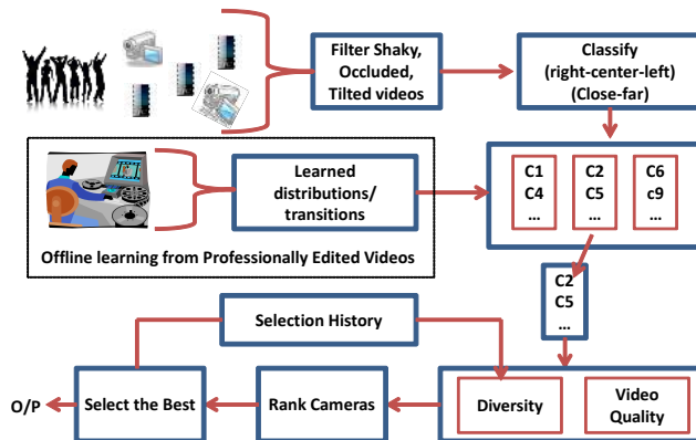
Figure 2: The virtual director framework
