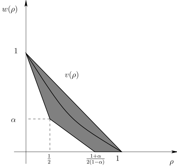
FIG. 3.1. Any w(\rho) with w(0) = 1 , w(1) = 0 and whose graph is in the grey region is admissible in Example 3.2 ( \alpha < 1/3 )
