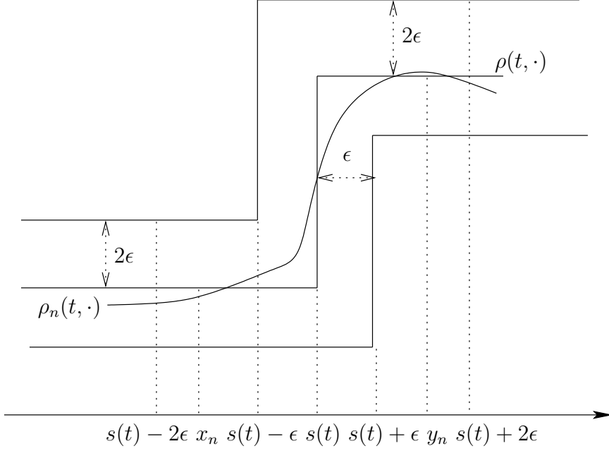
FIG. 4.1. Construction of the neighborhood for the graph of (the set-valued map) \rho(t, \cdot) close to a shock
