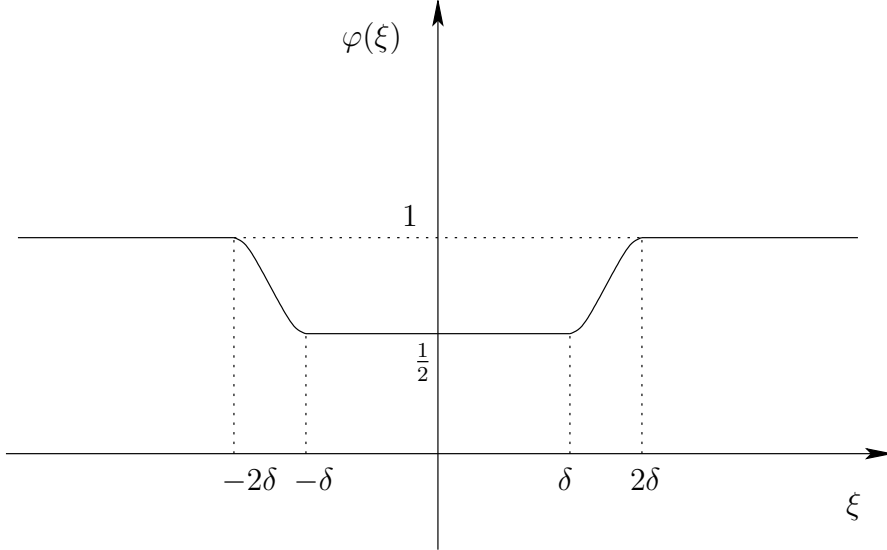
FIG. 2.1. An example of the cut-off function \varphi(\xi) with \beta = \frac{1}{2}
