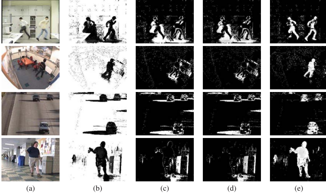
Figure 4. Sample visual results of detecting cast shadows in various environment. (a) Frame from video sequence. (b) Background posterior probability P(BG|x_p) . (c) Confidence map predicted by the global shadow model. (d) The shadow posterior probability P(SD|x_p) . (e) The foreground posterior probability P(FG|x_p) .
