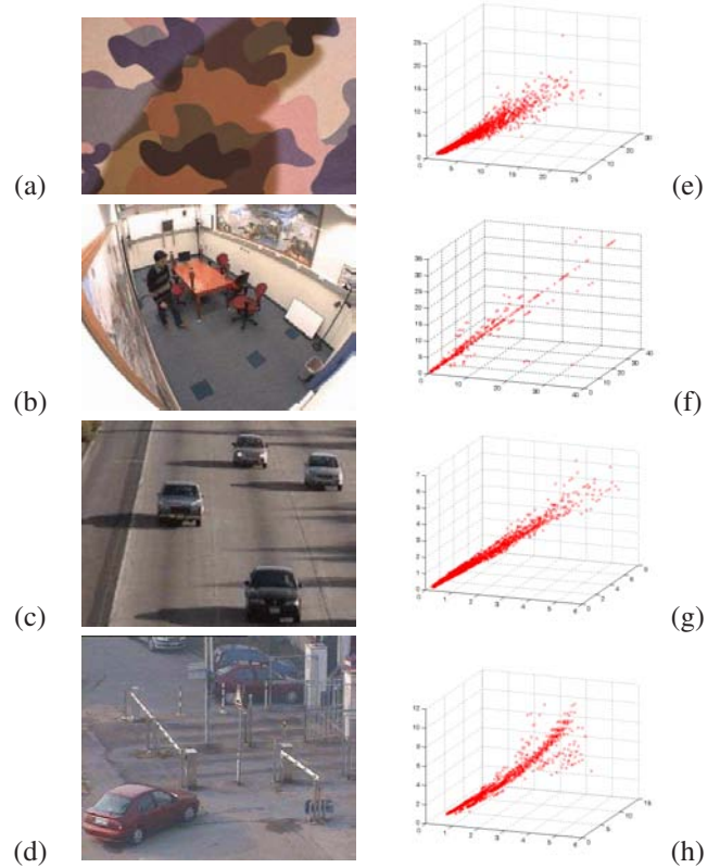
Figure 2. The color feature value distribution in various environments and illumination conditions. (a)-(d) Frame with cast shadows. (e)-(h) The corresponding feature value distribution in the S_1 S_2 S_3 space. Note that the feature values extracted from different background surface generally follow a line.
