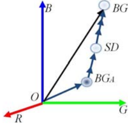
Figure 1. The contribution of all direct light sources and ambient illuminance. The shadow values SD are expected to be observed along the line between background value BG and the constant ambient term BG_A . Note that the shadow values do not necessary to be proportional to the direction of background values.
