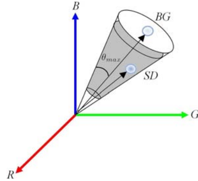
Figure 3. The weak shadow detector. The observation will be considered as potential shadow point if it falls into the gray area. The weak shadow detector contains three parameters: maximum allowed color shift, and minimal and maximal illumination attenuation.
