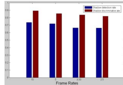
Figure 6. Quantitative results of the Intelligent Room sequence. Shadow detection and shadow discriminative rate are calculated under different frame rates settings.
