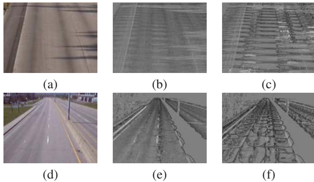
Figure 5. The effect of confidence-rated Gaussian mixture learning. The mean maps of local shadow model are taken at the 100 th frame (the first row) and 1000 th frame (the second row) (a)(d)The background image. (b)(e) The mean map of the most important Gaussian in the mixture with confidence-rated learning. (c)(f)The mean map without using confidence-rated learning.
