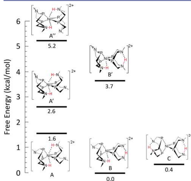
Figure 4. Ranking of the lowest free energy isomers of [Ni(P^{Cy_2}N^{Me_2}H)_2]^{2+} calculated in acetonitrile at the B3P86/ \{Ni(SDD);P,N,C,H(6-31G^*);(N)-H(6-31G^{**})\} level of theory. For clarity, cyclohexyl groups on the P atoms are not shown.
