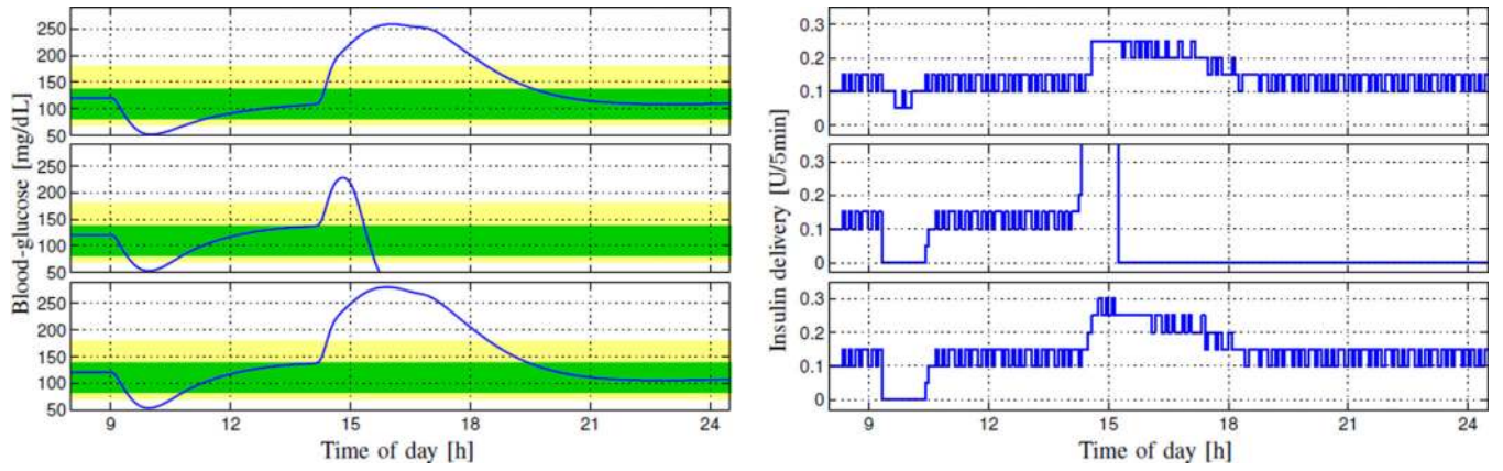
Fig. 1. Demonstration of asymmetric input cost function. Top: Symmetric, high cost, \hat{R} = \check{R} = 7000 . Middle: Symmetric, low cost, \hat{R} = \check{R} = 100 . Bottom: Asymmetric, \hat{R} = 7000 , \check{R} = 100 . Green area: [80, 140] mg/dL. Yellow area [70, 180] mg/dL.
