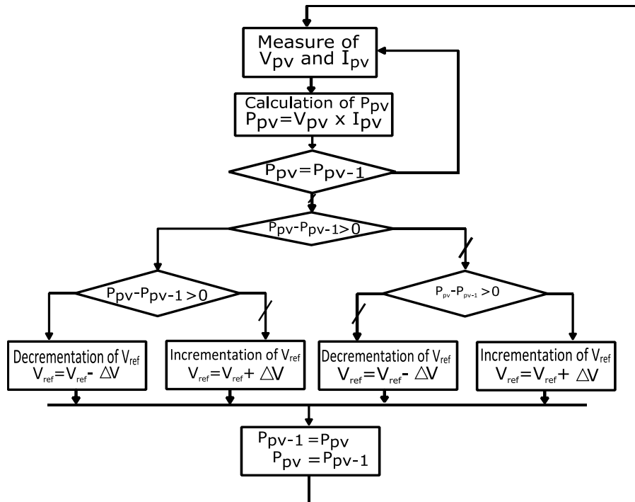
Figure. 4 Organization charts of P&O algorithm
