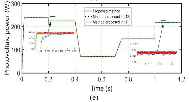
Figure. 8 PV module: a- current. b-Voltage. c-Power. Generated using the P&O, IC and the proposed controller. d – voltage and e – power of the proposed method compared to the ANN-Backstepping and ANN-ISMIC
