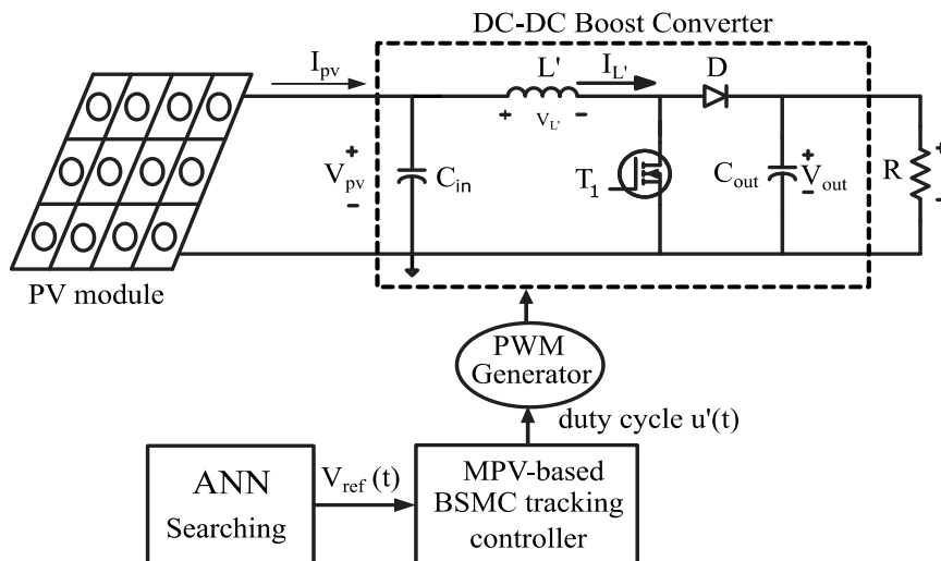
Figure. 1 Photovoltaic system
