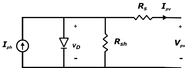
Figure. 2 Single diode PV cell
