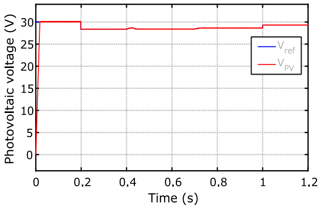
Figure. 7 The reference voltage generated by the ANN loop and the PV voltage using BSM loop
