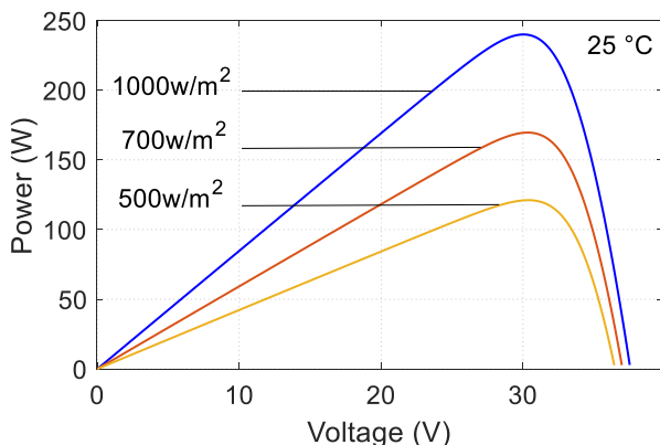
Figure. 3 Power-Voltage curves
