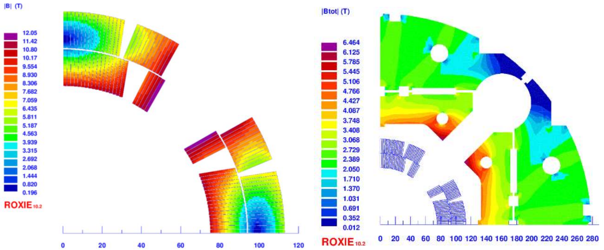
Fig. 3.7: Magnetic flux density in the coil (left) and in the yoke (right) at nominal current ( I_{nom} ).
