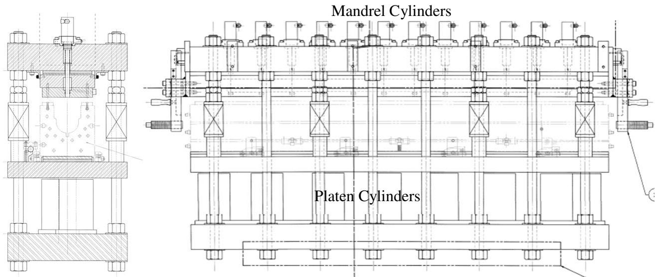
Fig. 4.6: Curing Press.
