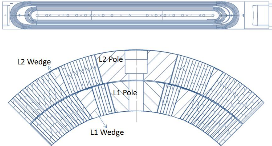
Fig. 4.2: MQXFS Coil Model.
