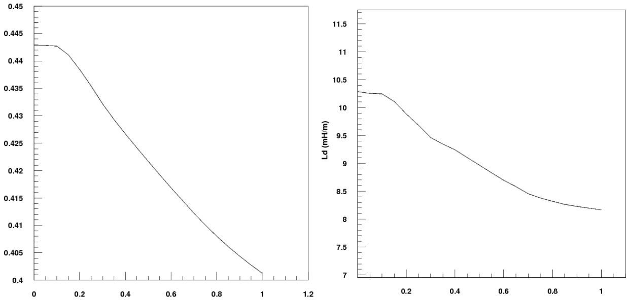
Fig. 3.8: Left: Transfer function defined as B_2(R_{ref}, I)/I and expressed in [T/kA] plotted versus I/I_{nom} . Right: differential inductance L_d in mH/m plotted versus I/I_{nom} . Roxie was used for the computations.
