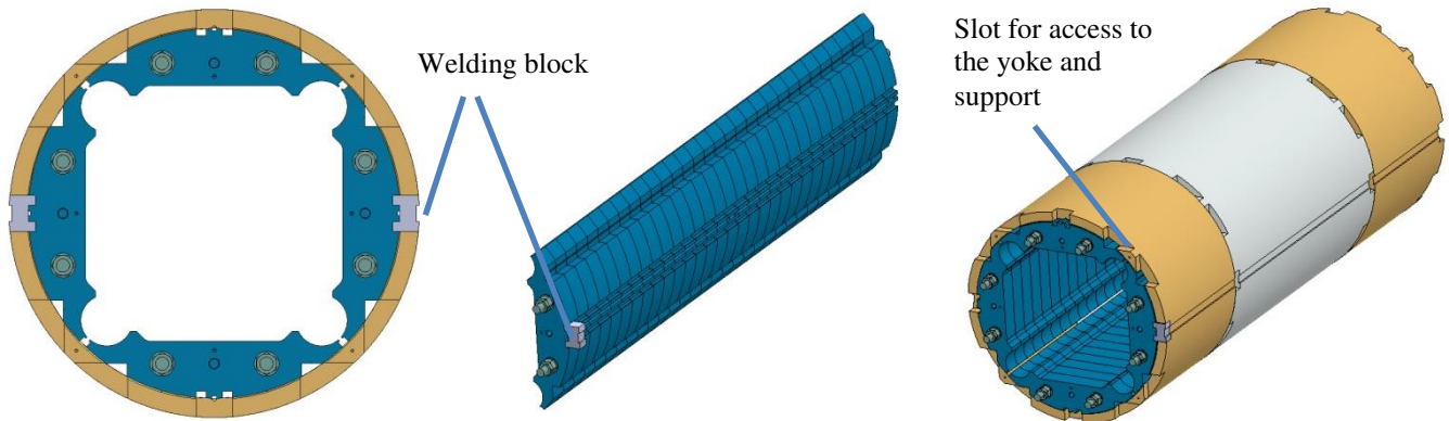
Fig. 6.2: Structure with features for welding the stainless steel shell.
