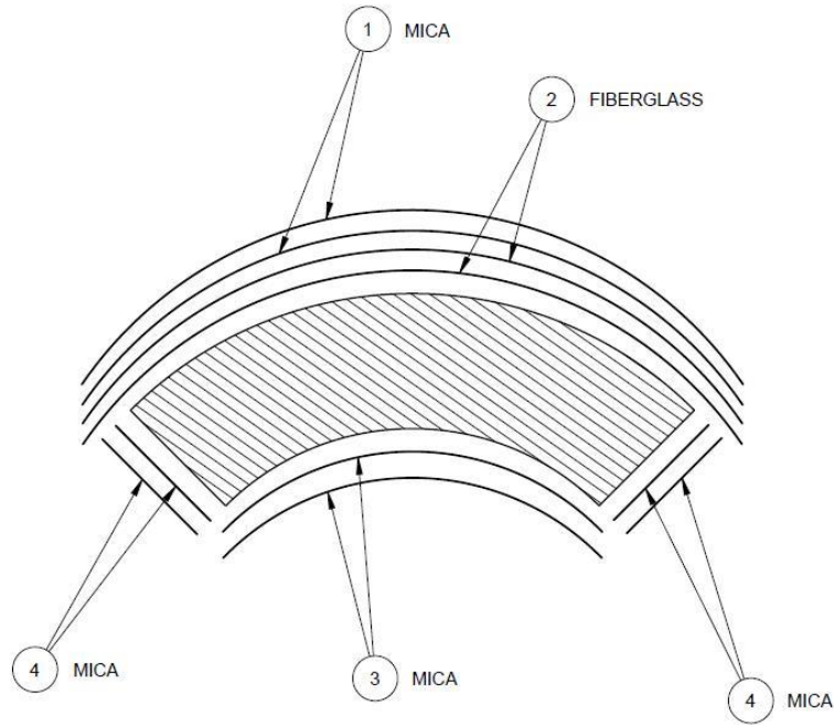
Fig. 5.2: Coil cross section during reaction.
