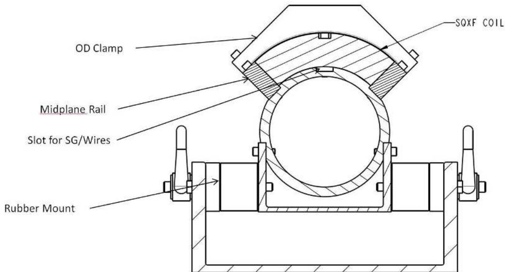
Fig. 5.4: Coil shipping fixture.
