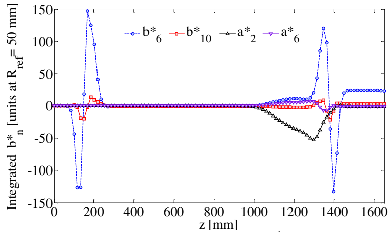
Fig. 3.17: Variation of the average multipole content in 10^{-4} units in the axial direction (from return end to lead end) computed by ROXIE. Multipoles computed at a reference radius of 50 mm for a magnetic length of 1.2 m (MQXFS).
