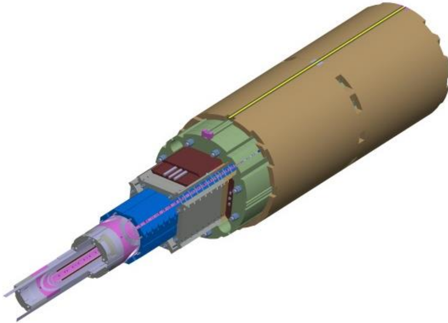
Fig. 6.3: Exploded view of the MQXFS1 structure (without axial load components and SS shell) showing in yellow the mid-plane backing strip (the magnet is shown here rotated by 90 degrees with respect to Fig. 6.1 and 6.2).
