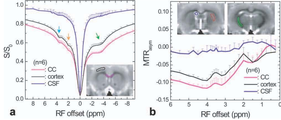
FIG. 2. a : The averaged Z-spectrum obtained at cortex, corpus callosum (CC), and cerebrospinal fluid (CSF) ROIs ( n = 6 ). b : MTR_{\text{asym}} shows CEST peaks at 3.6 and 2 ppm on top of the distorted negative background due to the MTC_{\text{IM}} asymmetry and NOE effects, which is more prominent in the CC ROI. Insets: three slices of S/S_0 map measured at 5.0 ppm from one representative animal, where the contours of cortex (black), CC (pink), caudate-putamen (red), internal capsule (green), and CSF (blue) ROI were depicted.
