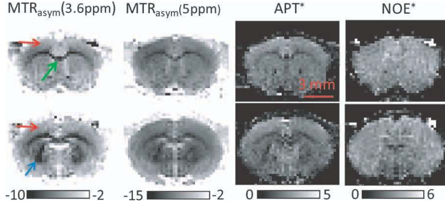
FIG. 5. In vivo maps of MTR_{\text{asym}}(3.6 \text{ ppm}) , MTR_{\text{asym}}(5 \text{ ppm}) , APT^* , and NOE^* were obtained from the rat brain for two slices. Note the two MTR_{\text{asym}} maps are negative and have similar tissue contrast, where cortex, CC, and IC areas are indicated by red, green, and blue arrows, respectively. The units here are % of S_0 .
