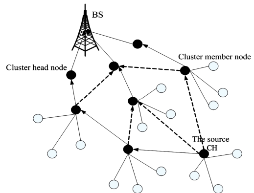
Figure 2. The net topology.
