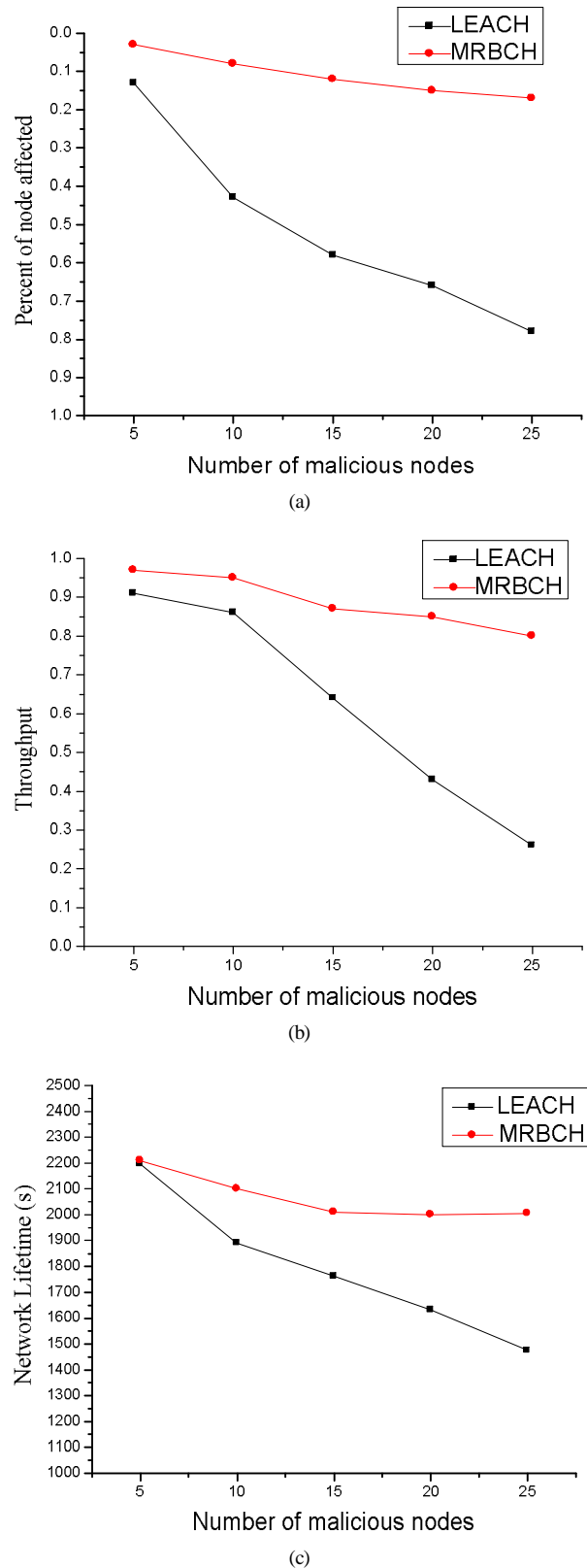
Figure 5. Comparing network performance between MRBCH and LEACH. (a) Average affected nodes; (b) Average network throughput; (c) Average network lifetime.
