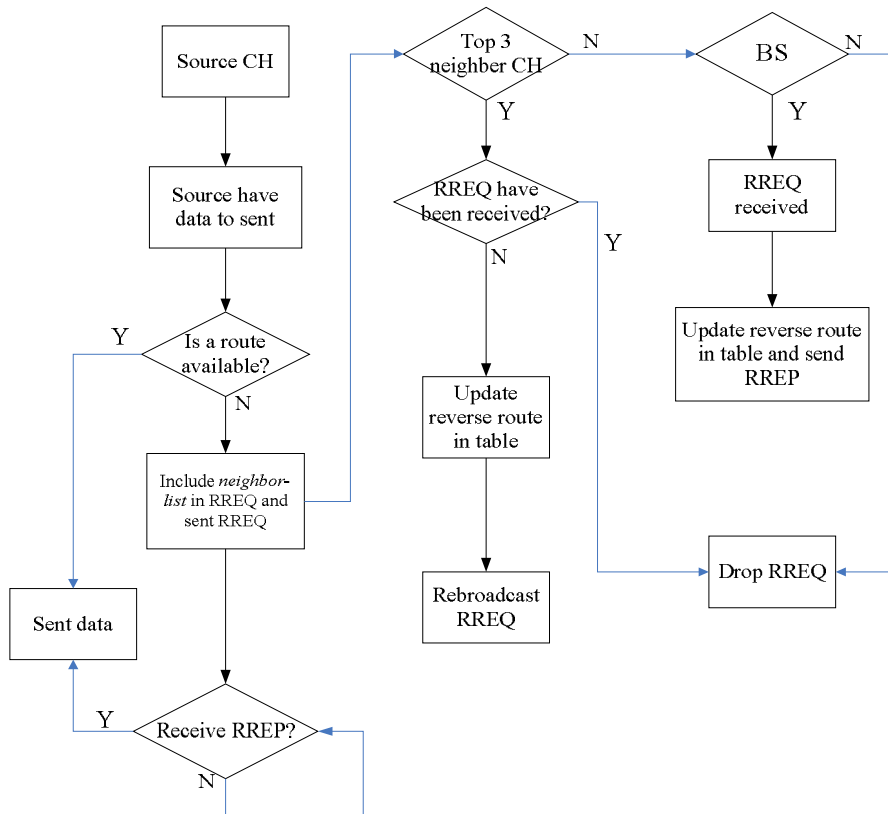
Figure 4. Route discovery process of MRBCH.
