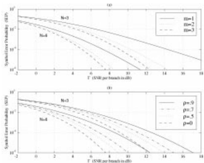
Fig. 1. The symbol error probability for QPSK with MRC as a function of the average SNR per branch for: (a) i.i.d. Nakagami channels with m = 1, 2 and 3; (b) identical Nakagami channels with exponential correlation where the correlation coefficient \rho = 0, 0.5, 0.7 and 0.9 with m = 3 .
