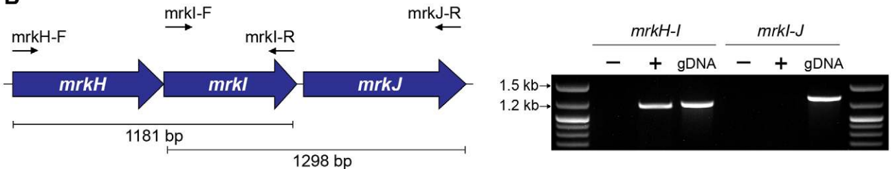
Figure 2. The mrkABCD and mrkHIJ loci in K. pneumoniae AJ218. (A) Genetic organization of the mrkABCD and mrkHIJ gene clusters from K. pneumoniae strains AJ218, NTUH-K2044 (GenBank Ref: AP006725), MGH 78578 (GenBank Ref: CP000647) and 342 (GenBank Ref: CP000964). (B) RT-PCR analysis of mrkHIJ transcription. PCR amplicon products of either RNA (–), reverse transcribed DNA (+) or genomic DNA (gDNA) were visualized on a 1% agarose gel. The mrkH-I product was generated with primer mrkI-R and amplified with primers mrkH-F and mrkI-R. The mrkI-J product was generated with primer mrkJ-R and amplified with primers mrkI-F and mrkJ-R. doi:10.1371/journal.ppat.1002204.g002
