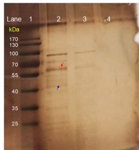
FIG 7 SDS-polyacrylamide gel image of the APCP-treated and untreated (control) MS2 viral surface proteins. The plasma was generated with the device used to test waterborne viruses, the plasma generation power was 28 W, and the time of exposure was 180 s. Lanes: 1, protein ladder; 2, untreated MS2 virus control; 3, plasma-treated MS2 viral proteins; 4, negative control (DI water). Red arrow, replicase protein (60 kDa); blue arrow, maturation protein (40 kDa).
