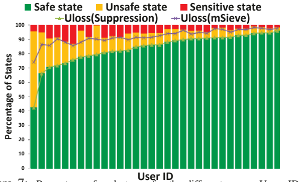
Figure 7: Percentage of node types for the different users. Users IDs are sorted in ascending order of safe node percentage. Privacy sensitivity \epsilon = 0.5 .
