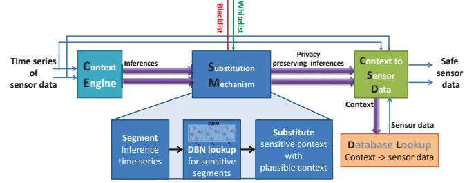
Figure 3: An overview of the mSieve framework.
