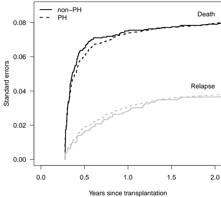
Figure 7: Standard errors for the transition probabilities AE \rightarrow Relapse and AE \rightarrow Death (starting time: 100 days), both for the full model and the proportional hazards model
