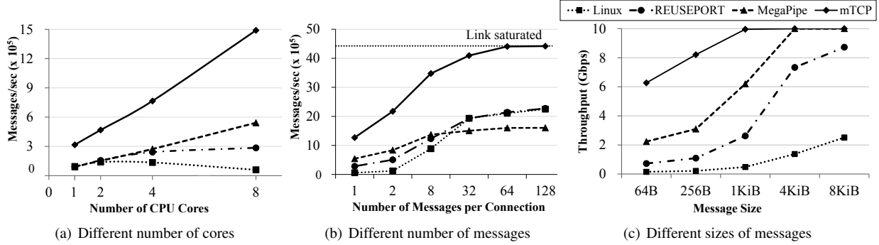
Figure 7: Performance of short TCP connections with 64B messages. (a) and (c) use one message per connection.
