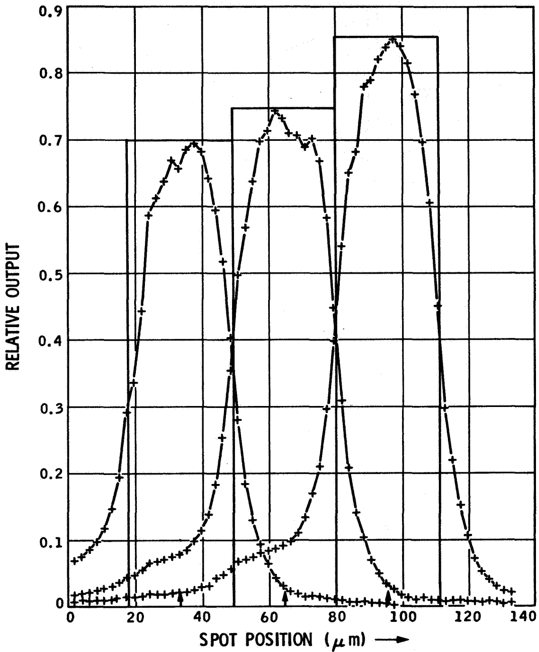
Figure 12. Sensitivity profile for three adjacent pixels (blue filter) (scan || to vertical channel)
