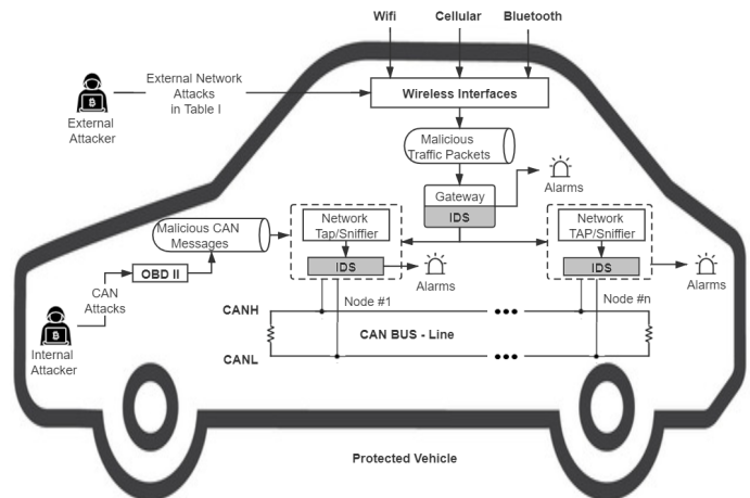
Fig. 2. The proposed IDS-protected vehicle architecture.
