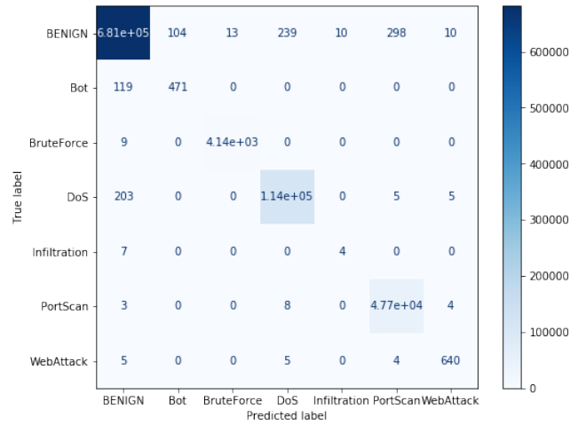
Fig. 5. Confusion matrix for the test set of CICIDS2017 dataset.
