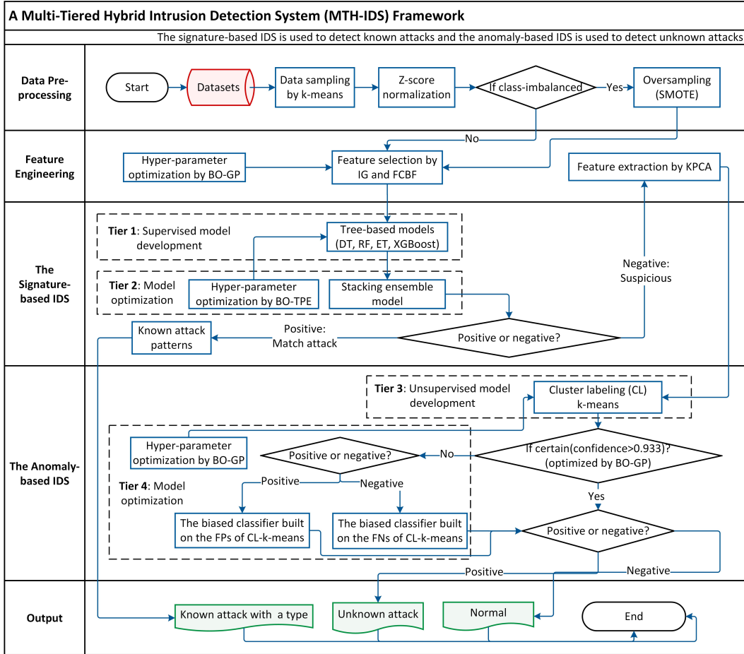
Fig. 3. The framework of the proposed MTH-IDS.
