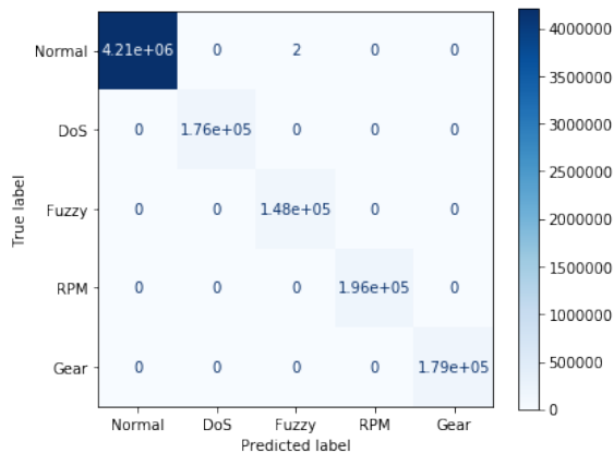
Fig. 4. Confusion matrix for the test set of CAN-intrusion-dataset.
