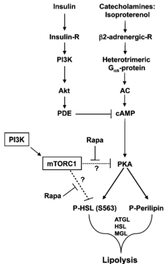
Fig. 6. Model for the role of mTORC1 signaling in suppression of lipolysis in adipocytes. The \beta -adrenergic agonist isoproterenol, a synthetic catecholamine, promotes triacylglycerol (TAG) breakdown (lipolysis) by activating a large heterotrimeric G αs -protein that activates adenylate cyclase (AC), which converts ATP into cAMP. cAMP binds the regulatory subunits of protein kinase (PKA), thus dissociating the repressive regulatory subunits from the catalytic subunits. Catalytically active PKA phosphorylates downstream targets, including perilipin and hormone sensitive lipase (HSL), which contribute to initiation of lipolysis together with several other lipases including ATGL (adipose triacylglycerol lipase) and MGL (monoacyl lipase), ultimately leading to the breakdown of TAG into free fatty acids (FFA) and glycerol. mTORC1 signaling suppresses lipolysis by either acting on common lipolytic targets (e.g., HSL, others?) via a pathway parallel to PKA or by converging on PKA to inhibiting its function. By inhibiting mTORC1 signaling, rapamycin synergizes with the PKA pathway to promote lipolysis, thus reducing TAG storage; therefore, mTORC1 signaling suppresses lipolysis, thus augmenting TAG storage
