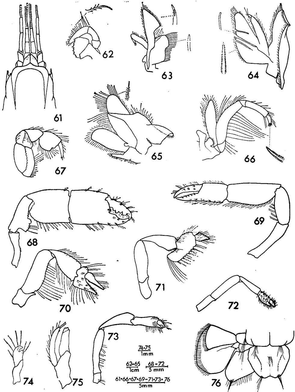
Callinassa guara , sp. n. 61, anterior part of body in dorsal view; 62, mandible; 63, maxillula; 64, maxilla; 65, first maxilliped; 66, second maxilliped; 67, third maxilliped; 68, larger first leg of male; 69, smaller first leg of male; 70, second leg; 71, third leg; 72, fourth leg; 73, fifth leg; 74, first pleopod of male; 75, second pleopod of male; 76, telson and left uropod in dorsal view.
