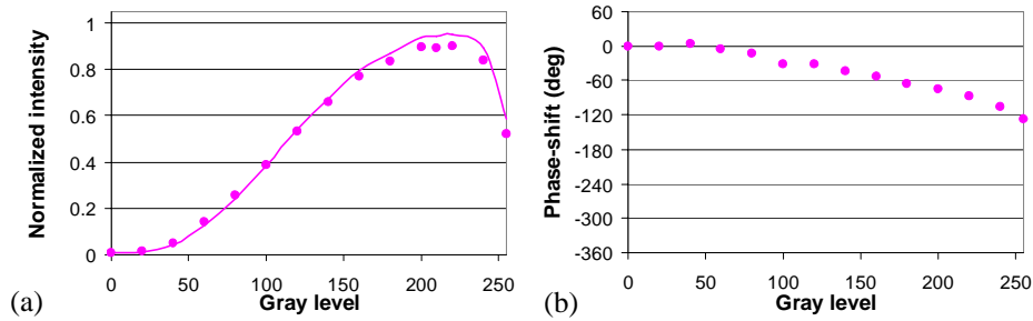
Fig. 8. Maximum intensity contrast. (a). Normalized intensity (theory – line, experiment – symbols). (b). Phase-shift (experimental). Configuration given in Table 1. The low phase-shift depth enables to use this configuration for amplitude-mostly modulation.
