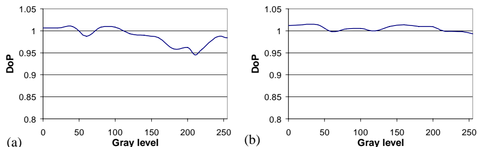
Fig. 14. Theoretical DoP for the SOP reflected by the LCoS. In (a) for the incident SOP used in Fig. 11, and in (b) for the incident SOP used in Fig. 12.
