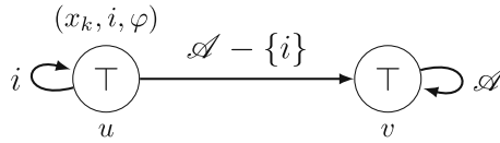
Fig. 31 The update frame \text{PRI}_i^{(k, \varphi)}
